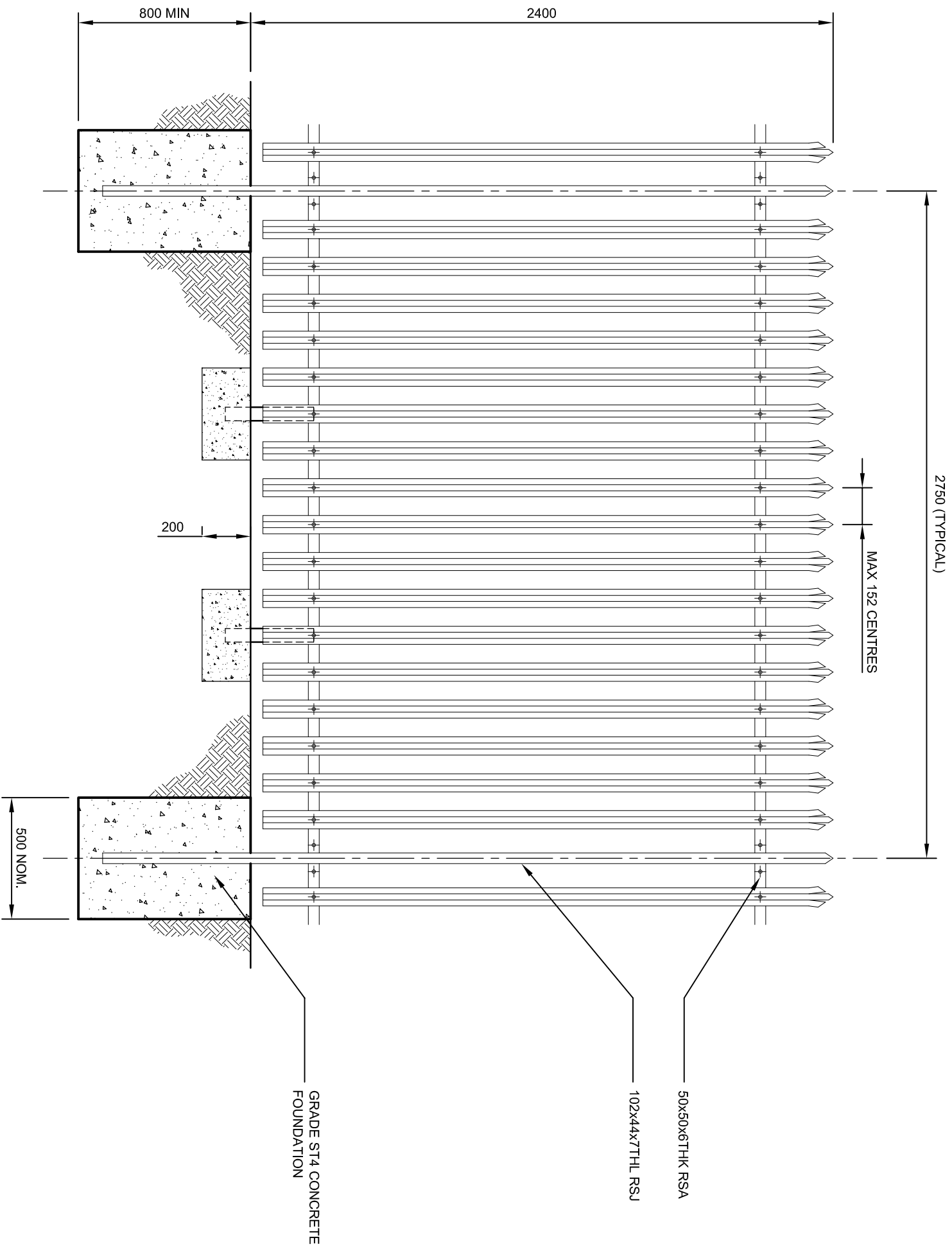
TYPICAL PALISADE FENCE PANEL - SECURITY PURPOSE GRADE
